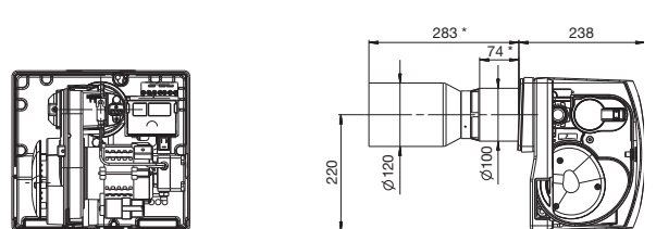
Unit flange
